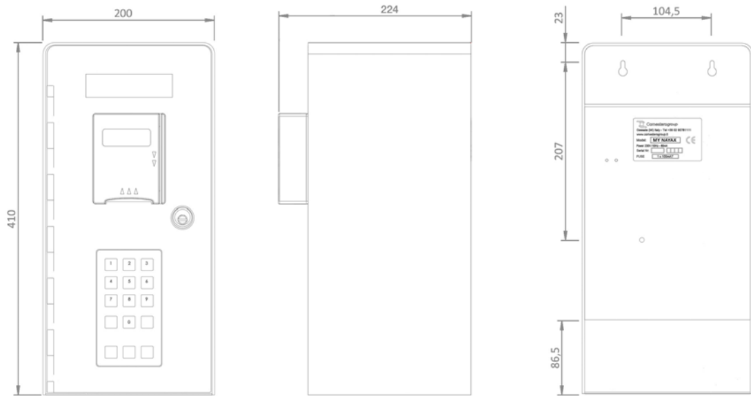
Technical Schematics NOTE: UNIT OF MEASURE MM
